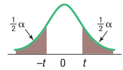
Two-tailed test
